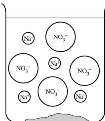
Solid \text{PbI}_2
