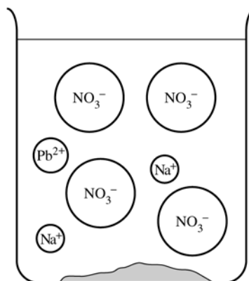
Solid \text{PbI}_2
