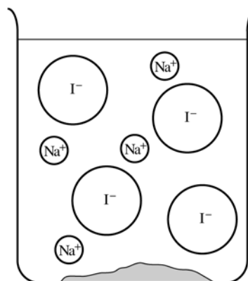
Solid \text{Pb}(\text{NO}_3)_2
