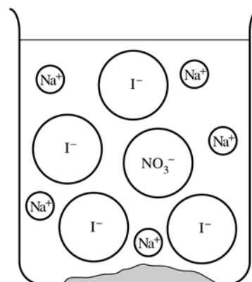
Solid \text{PbI}_2
